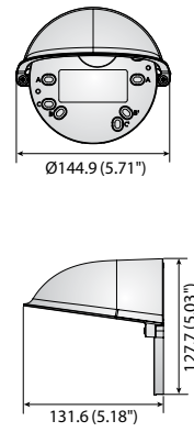
SBV-120WC
