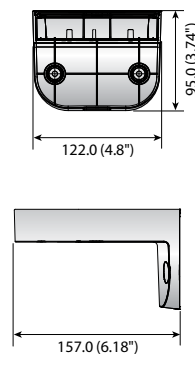
SBP-300WM0/120WM
