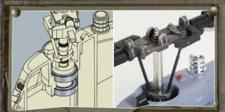
Dual-metal ball bearing rotor structure
