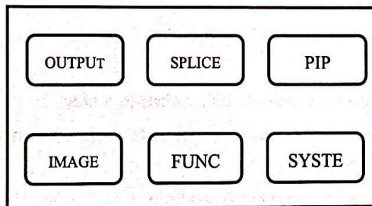
Figure12-Main menu
