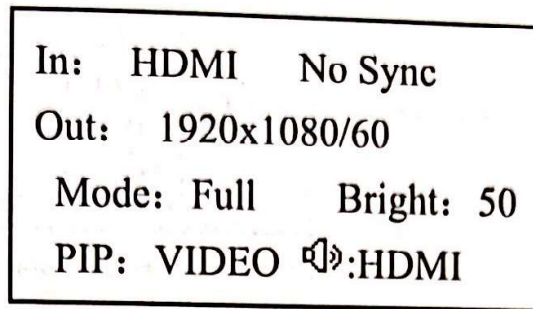
Figure 9 - Default menu
