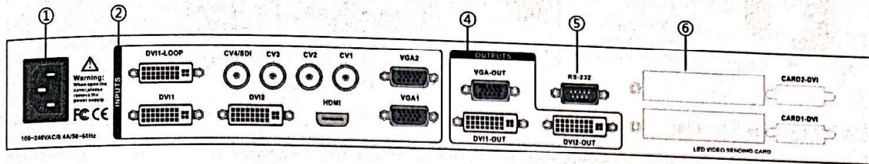
Figure 1-Video processor rear panel
