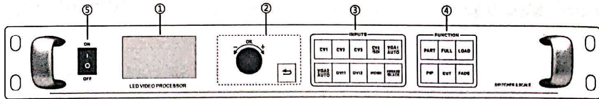
Figure 4-Front Panel
