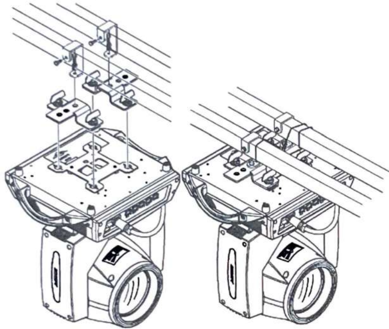
Figure 2 Installation
