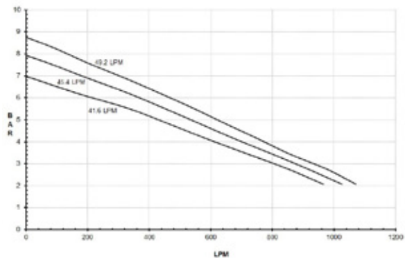
9306C-HM3C-3U & 9306S-HM3C-3U METRIC
