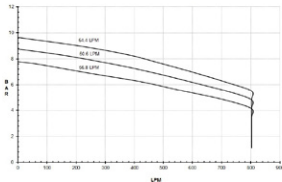
9306C-HM5C & 9306S-HM5C METRIC 9306C-HM5C-U & 9306S-HM5C-U
