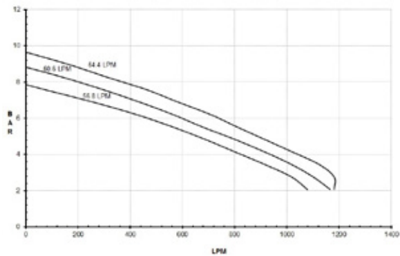
9306C-HM5C-3U & 9306S-HM5C-3U METRIC
