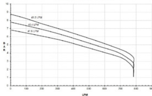
9306C-HM1C & 9306S-HM1C METRIC 9306C-HM1C-U & 9306S-HM1C-U
