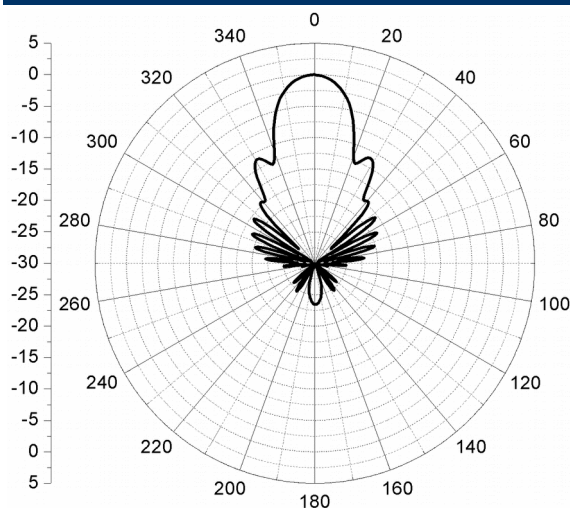
Diagrama de Radiação @860 MHz Plano – H Radiation Pattern @860 MHz – H Plane
