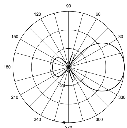
Diagrama de Radiação @860 MHz Plano – H Radiation Pattern @860 MHz – H Plane
