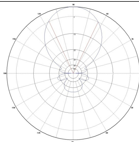
Diagrama de Radiação @455 MHz Plano – H Radiation Pattern @455 MHz – H Plane
