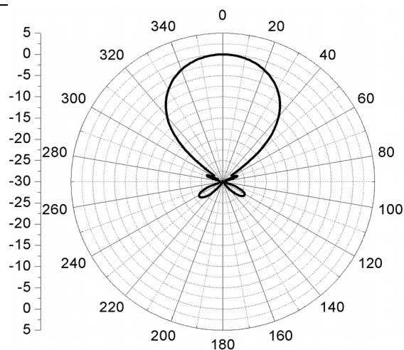
Diagrama de Radiação @380 MHz Plano – H Radiation Pattern @380 MHz – H Plane
