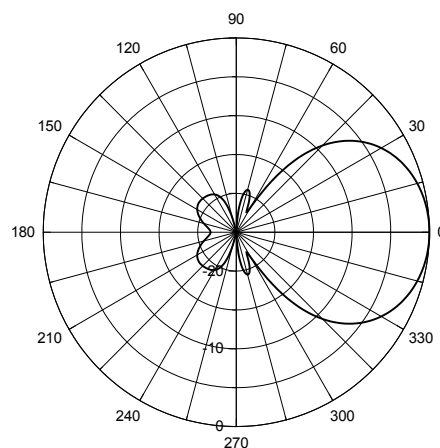
Diagrama de Radiação @ 1920 MHz Plano – H Radiation Pattern @ 1920 MHz – H Plane
