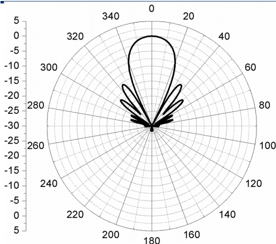
Diagrama de Radiação @1795 MHz Plano - H Radiation Pattern @1795 MHz – H Plane
