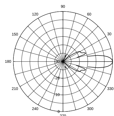
Diagrama de irradiação @ 925 MHz Plano Vertical Vertical Plane Radiation Pattern @ 925 MHz
