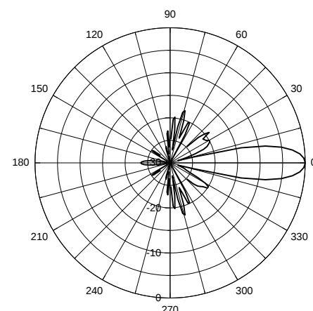
Diagrama de irradiação @ 860 MHz Plano Vertical Vertical Plane Radiation Pattern @ 860 MHz
