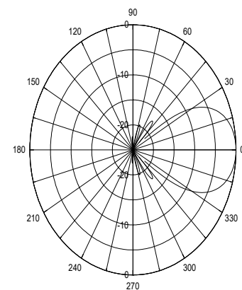
Diagrama de Radiação @1920 MHz Plano – H Radiation Pattern @1920 MHz – H Plane
