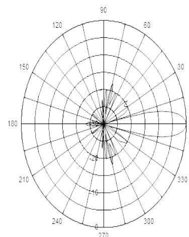
Diagrama de irradiação @ 860 MHz Plano Vertical Vertical Plane Radiation Pattern @ 860 MHz
