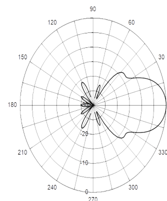
Diagrama de Radiação @860 MHz Plano – H Radiation Pattern @860 MHz – H Plane
