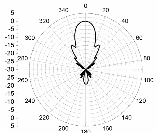
Diagrama de Radiação @830 MHz Plano – H Radiation Pattern @830 MHz – H Plane
