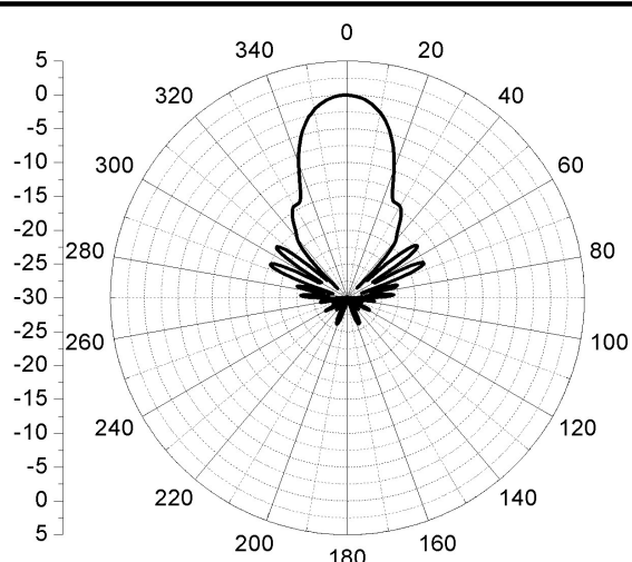
Diagrama de Radiação @740 MHz Plano – H Radiation Pattern @740 MHz – H Plane
