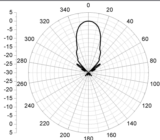
Diagrama de Radiação @740 MHz Plano – H Radiation Pattern @740 MHz – H Plane
