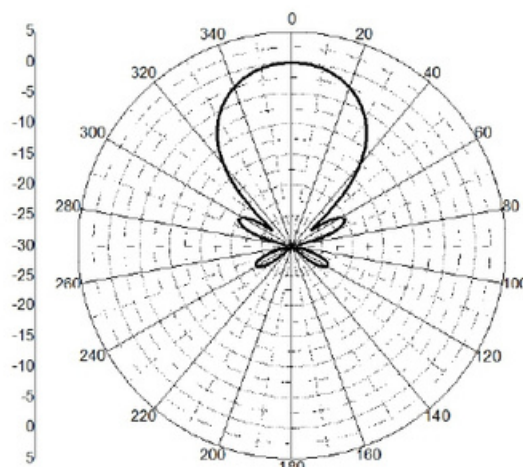
Diagrama de Radiação @420 MHz Plano – H Radiation Pattern @420 MHz – H Plane
