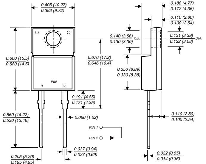
ITO-220AC (MBRF16xx)
