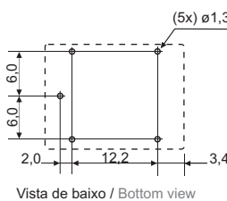
Diagrama PCI / Printed circuit layout
